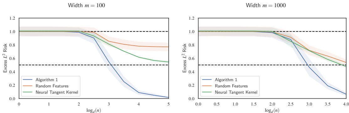
Figure 1: Sample Complexity: The x axis plots \log_d(n) and the y axis plots the excess risk in L^2(\mathcal{D}) for each of three methods: Algorithm 1, random features, and the neural tangent kernel. The top dashed horizontal line is at L^2 = 1 , which corresponds to outputting the zero predictor. The middle horizontal line is at L^2 = \frac{1}{2} and corresponds to learning the optimal quadratic predictor \frac{1}{2}He_2(x_1) . Due to its improved sample efficiency, Algorithm 1 easily achieves near zero excess risk despite the relatively high degree of f^* , while random features and the neural tangent kernel are only able to learn the optimal quadratic predictor. See Section 6 for additional experimental details.
