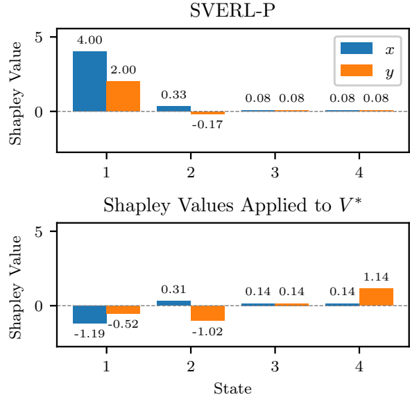
Figure 4. Shapley values of x and y state features in Gridworld-B. Top panel: SVERL-P. Bottom panel: Shapley values applied to a value function.
