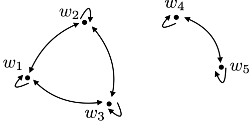
Figure 1: An S5 Kripke frame (W, R) on 5 possible worlds.
