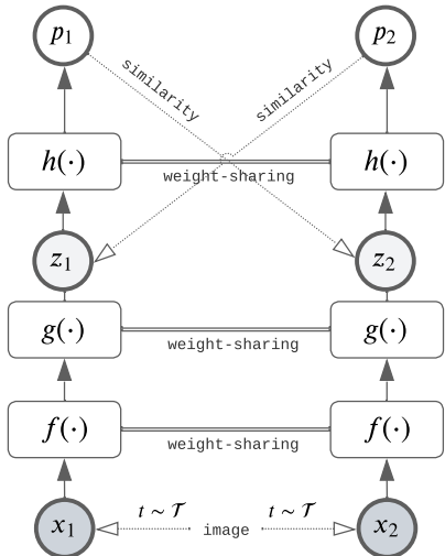
Figure 1: SimSiam architecture.
